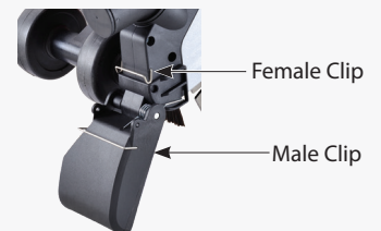
Spring-Loaded Splash Guard
