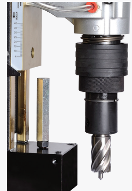
Annular Cutter Arbor (Annular cutter and pilot pin not included)
